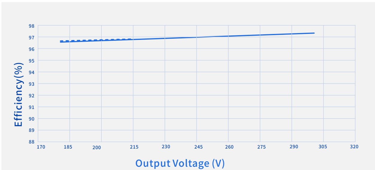
Efficiency Vs. Output Voltage ( V_{in}=347Vac )
